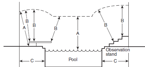
Figure 680.8 Clearances from Pool Structures.
